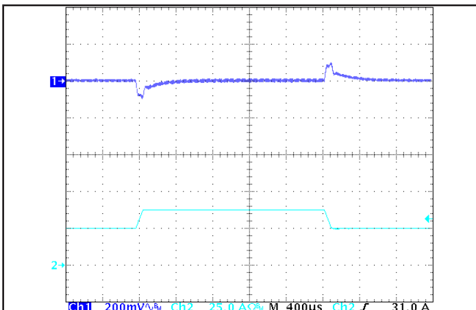
Figure 5: Output voltage response to step-change in load current (50 % -75 % -50 % of I_{out(max)} ; dI/dt = 0.1 A/\mu s ). Load cap: 15 \mu F tantalum cap and 1 \mu F ceramic cap. Ch 1: V_{out} , Ch 2: I_{out} .
